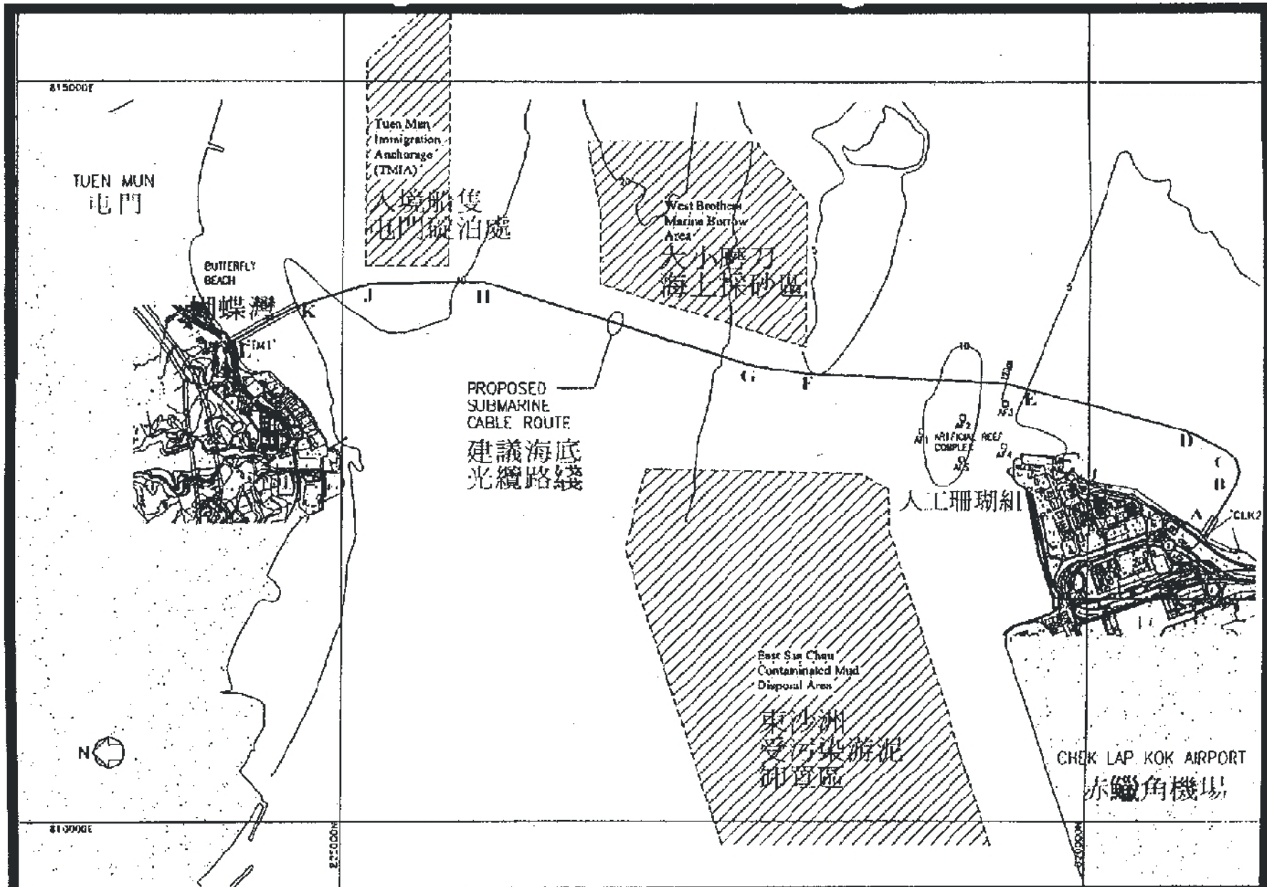
Figure 1 圖 1 Submarine Cable Landing Installation at Tuen Mun for HGC Optical Fibre Submarine Cable System between Tuen Mun and Chek Lap Kok 屯門至赤鱓角之和記海底纜系統屯門登岸段光纜鋪設工程
